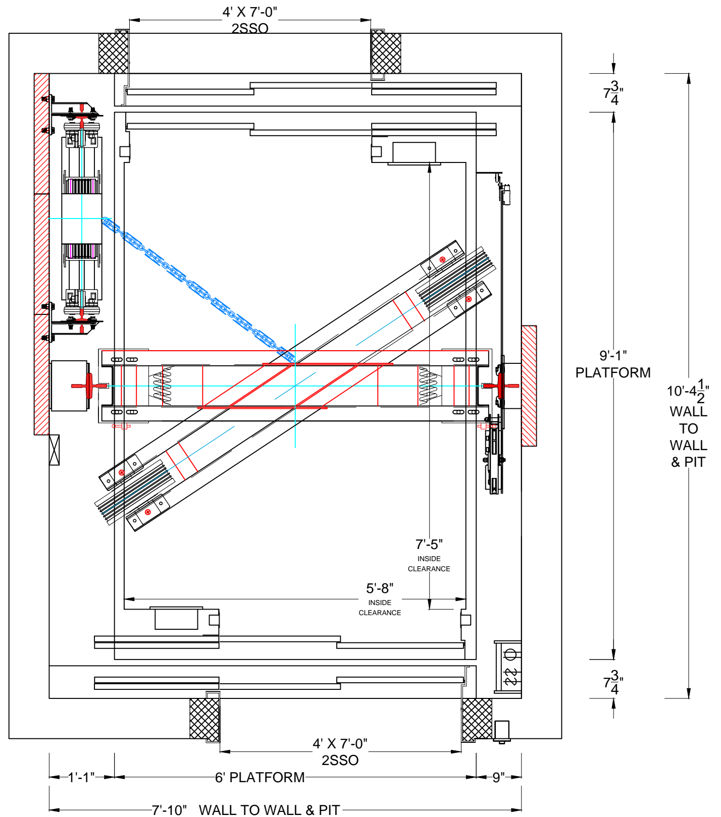
MRL 4,500 SERVICE FRONT ONLY BLDG SUPPORTED DIMENSIONS SHOWN ARE FOR SEISMIC ZONE 2 OR GREATER
