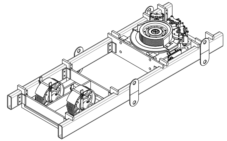
OVERHEAD MACHINE DETAIL FOR REFERENCE ONLY CAPACITY - UP TO 3,500 LBS SPEED - UP TO 350 FPM
